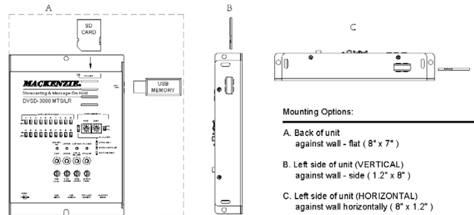
Figure 1 - Mounting
